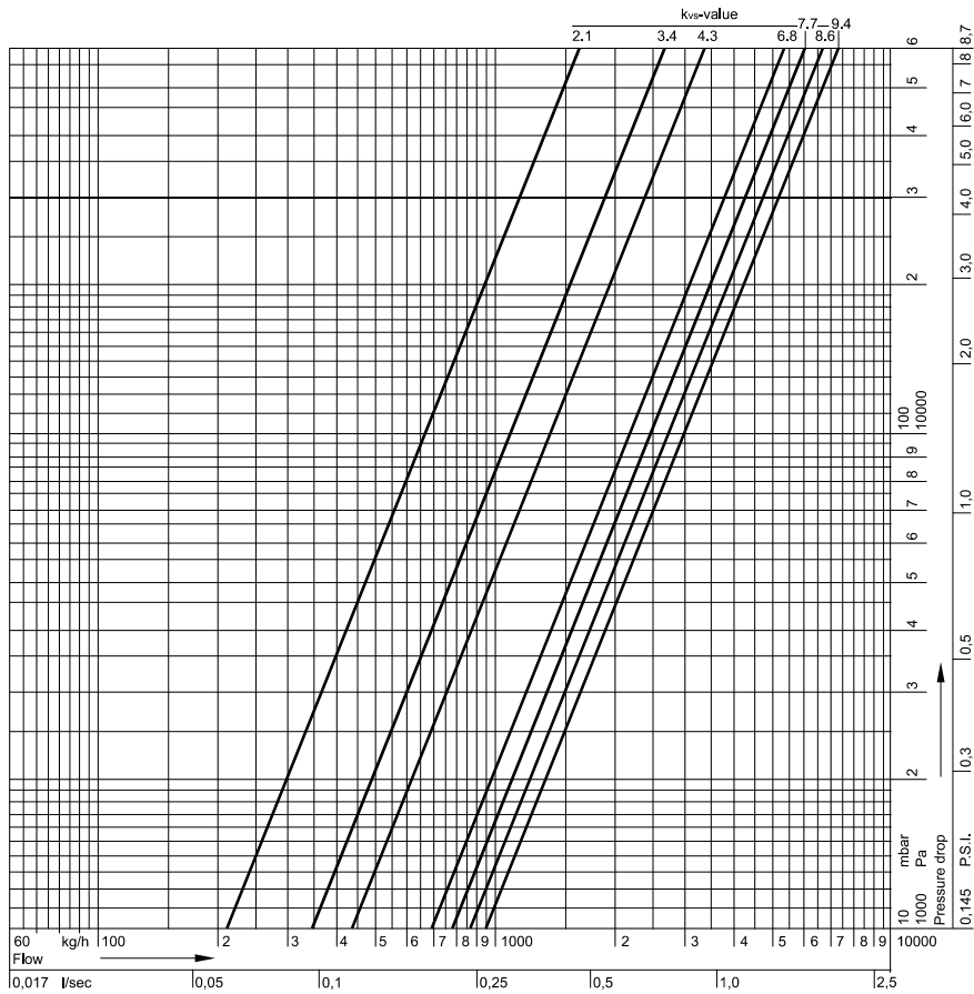
Fig. 9. Valve pressure loss characteristic
